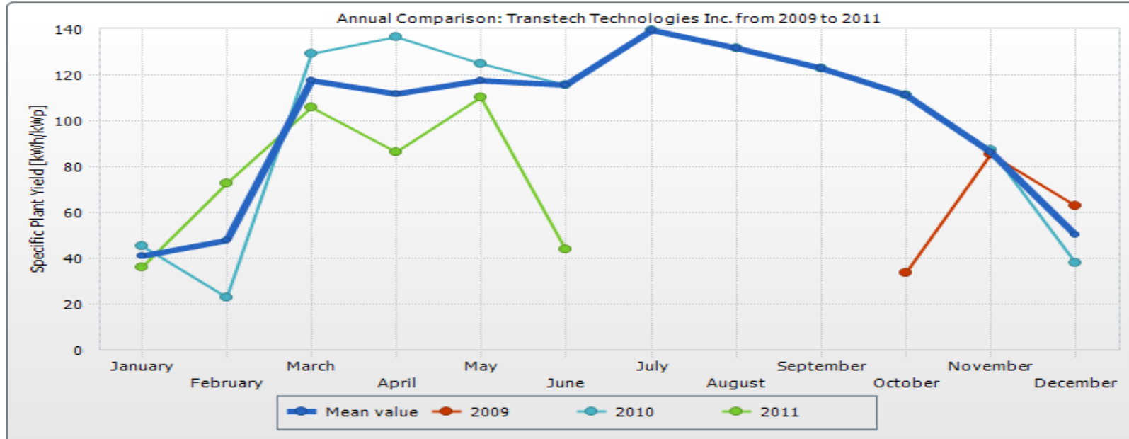
Specific Plant Yield [kWh/kWp]
